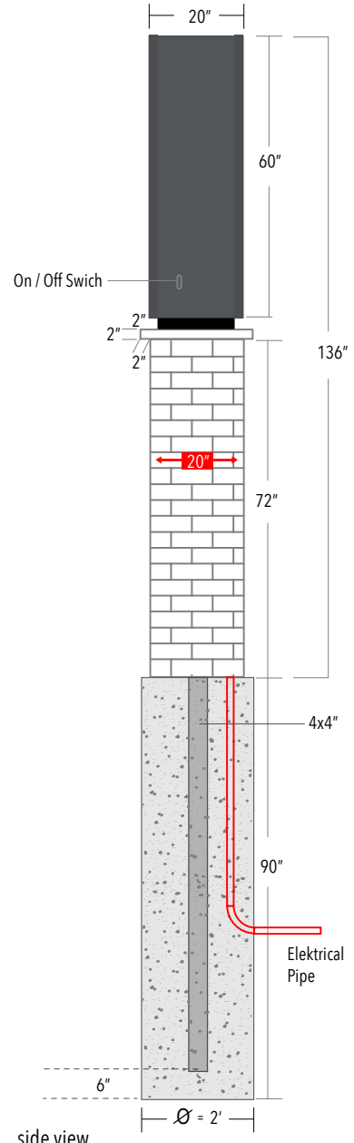
side view
